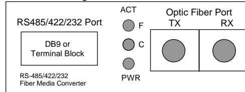
Fig. 6 RS-485/422/232 to ST Fiber Converter Front Panel
