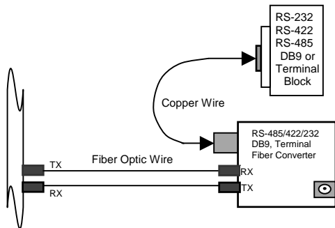
Fig. 5 RS-485/422/232 Fiber Optic Network Connection
