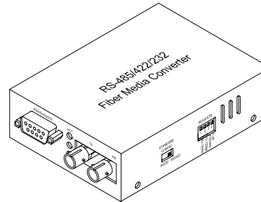
Fig. 1 RS-485/422/232 DB9 to Fiber Converter
